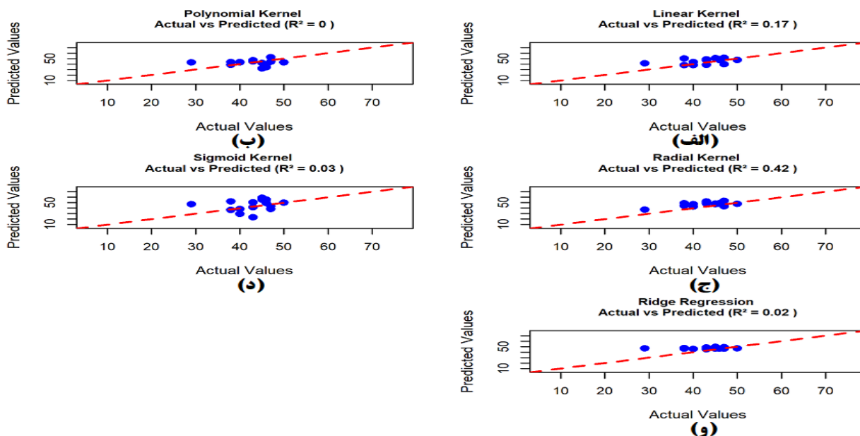
Actual vs Predicted Values In Region 2 [ca020]
