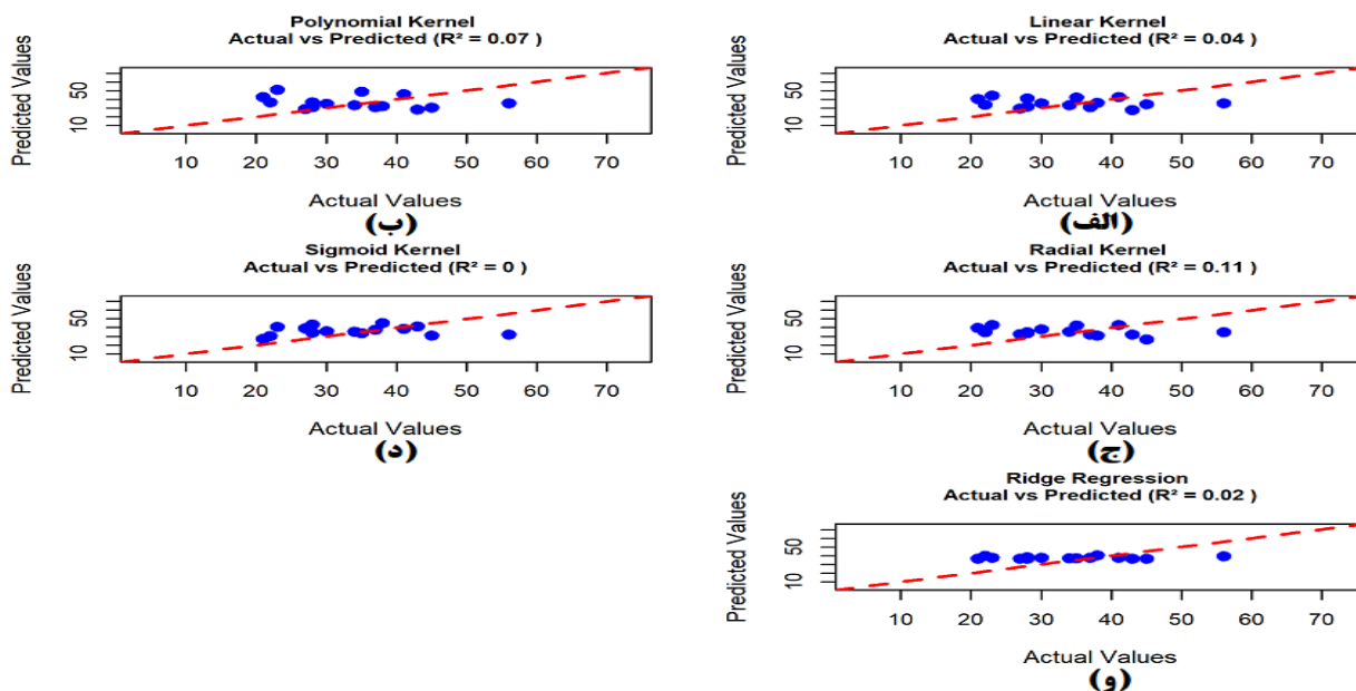
Actual vs Predicted Values In Region 2 [ca2040]
