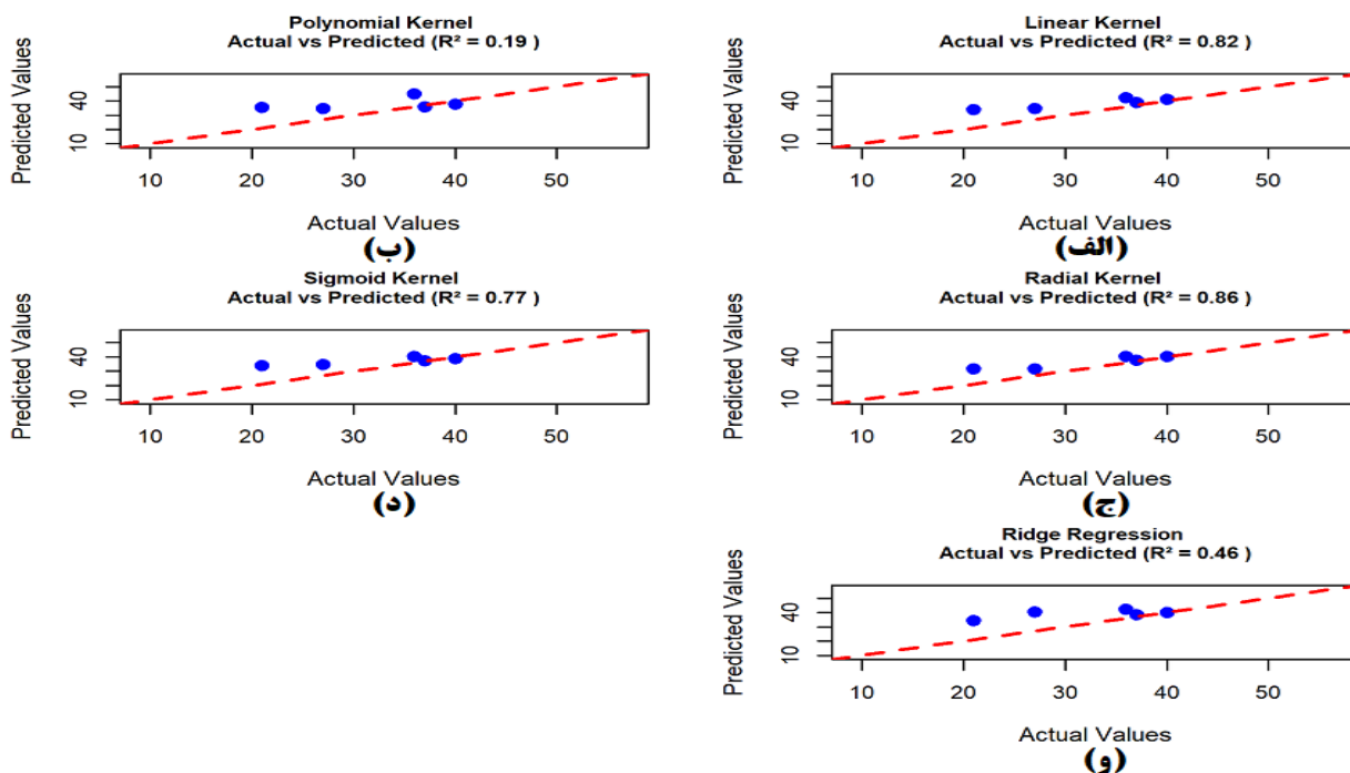
Actual vs Predicted Values In Region 1 [ca2020]
