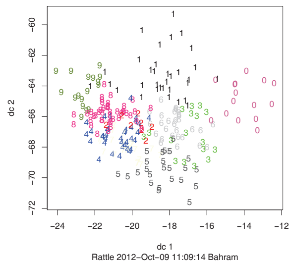
Discriminant Coordinates weather.csv
